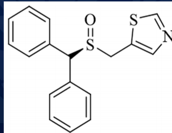
FIGURE 1 | Structure of the novel atypical dopamine reuptake inhibitor (S)-CE-123 ((S)-5-((benzhydrylsulfinyl)methyl)thiazole).
